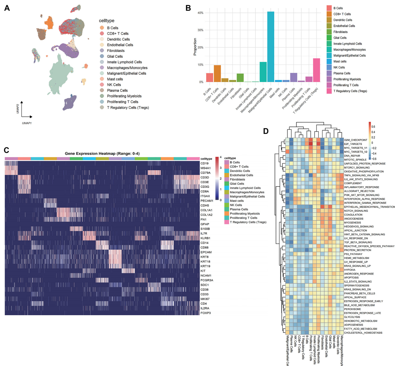
Figure 2. Overview of various cell types in the TME of CRC at the scRNA transcriptome level. (A) Identification of 15 cell types in 204 CRC tumor center tissues; (B) Bar plot showing the distribution proportion of each cell type; (C) Heatmap showing the expression distribution of classic marker genes for each cell type; (D) ssGSEA score from hallmark gene sets of Human MSigDB Collections, changes in the heatmap cell colors indicate the level of activity of the corresponding pathways in specific cell types. Abbreviations: CRC: Colorectal cancer; TME: Tumor microenvironment.
