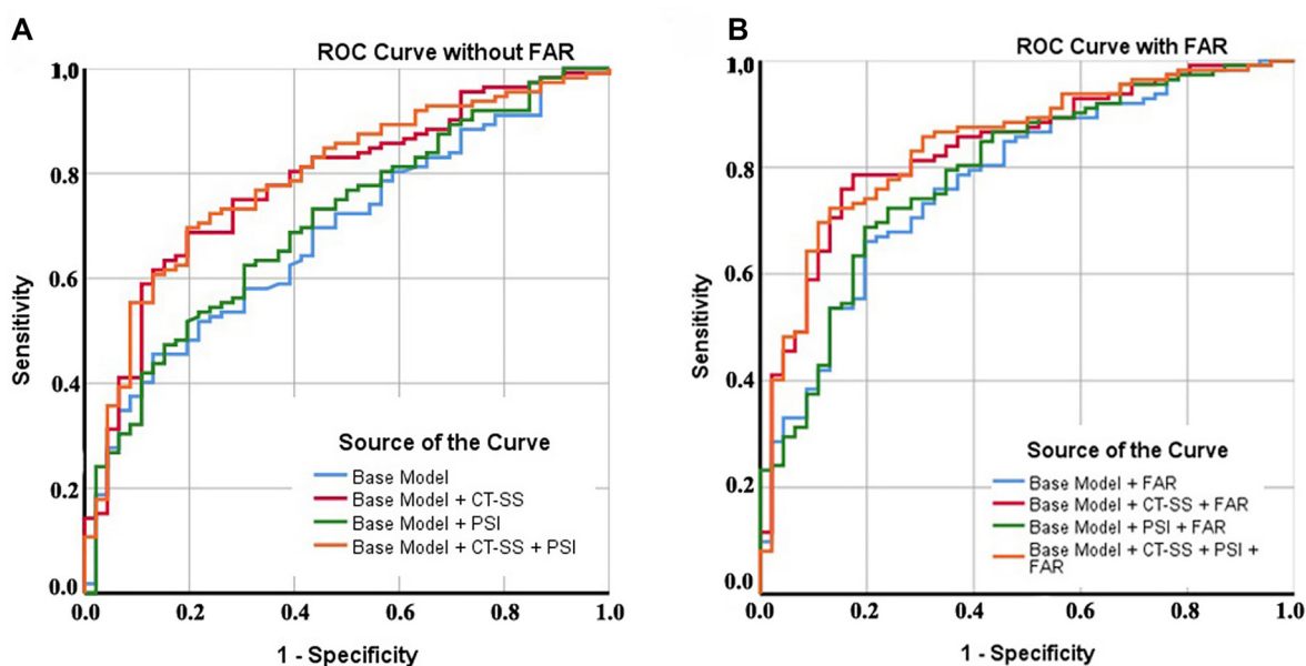
Figure 2. Comparison of ROC Curves based on various predictive models with and without FAR. (A) Without FAR; (B) With FAR. FAR: Fibrinogen-to-albumin ratio; CT-SS: Computed tomography severity scores; PSI: Pneumonia severity index; ROC: Receiver operating characteristic.
